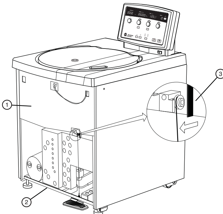
Figure 3.2 Manual Door Release
